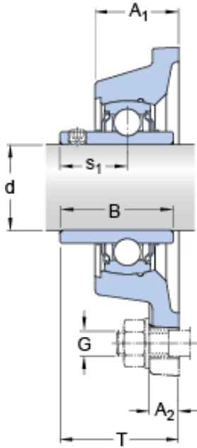
FY 1.15/16 TF/VA228 Bearing 2D drawings and 3D CAD models
